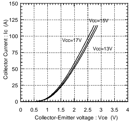
Collector current vs. Collector-Emittter voltage (typ.) Tj=25°C(Terminal)
