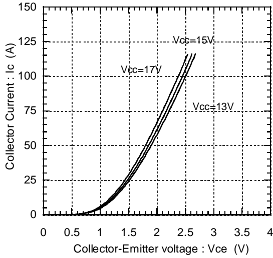
Collector current vs. Collector-Emittter voltage (typ.) Tj=25°C(Chip)
