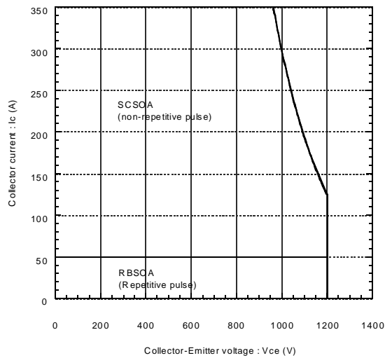
Reversed biased safe operating area V_{cc}=15V, T_j=25^\circ C (min.)
