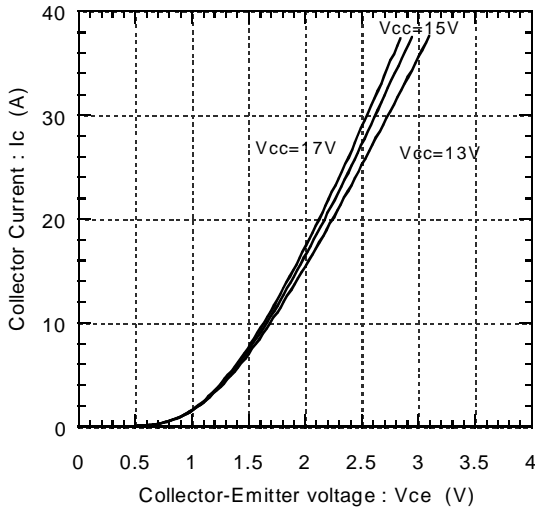
Collector current vs. Collector-Emmitter voltage (typ.) Tj=25°C
