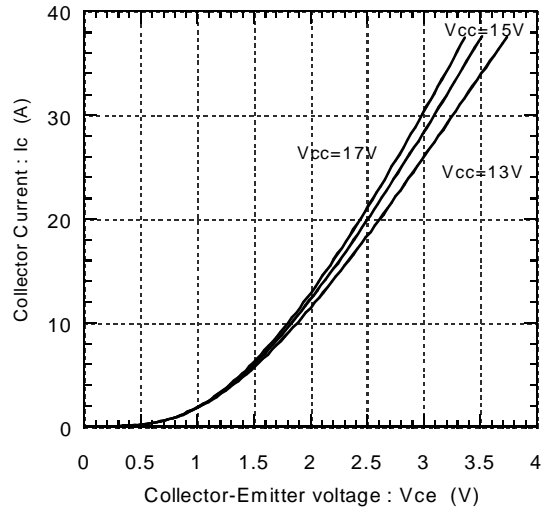
Collector current vs. Collector-Emmitter voltage (typ.) Tj=125°C
