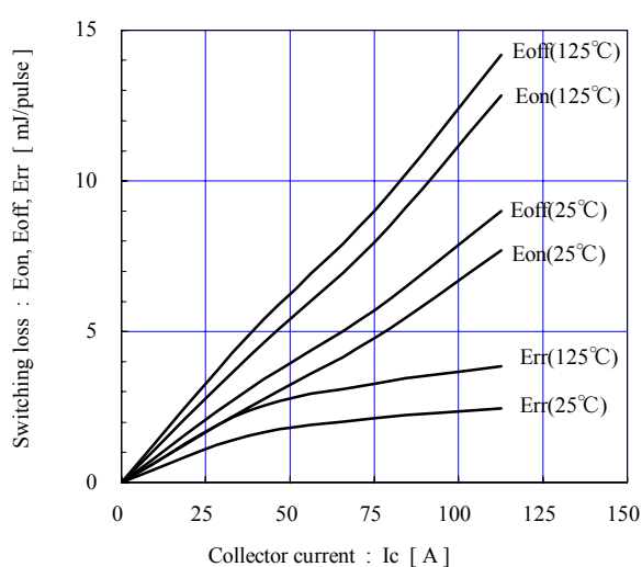
Switching loss vs. Collector current (typ.) V_{cc}=600V, V_{GE}=\pm 15V, R_g=9.1\Omega
