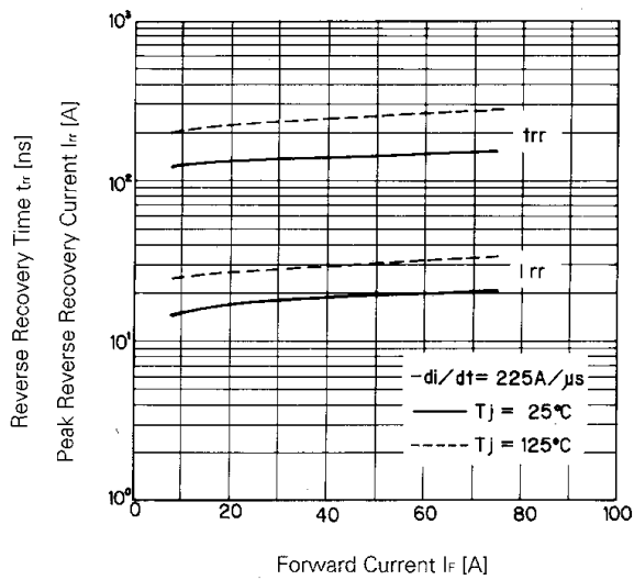
T_{rr}, I_{rr}-I_F
