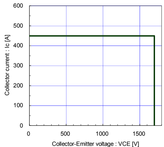
Reverse bias safe operating area (max.) +V_{GE}=15V, -V_{GE} \le 15V, R_g \ge 2.2\Omega, T_j \le 125^\circ C Stray inductance \le 100nH
