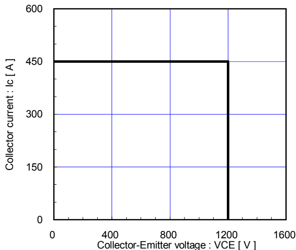
Reverse bias safe operating area (max.) +V_{GE}=15V, -V_{GE} \le 15V, R_G \ge 3.0\Omega, T_j \le 125^\circ C Stray inductance \le 100nH
