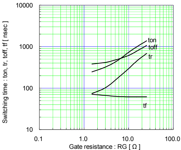
Switching time vs. Gate resistance (typ.) V_{cc}=600V, I_c=225A, V_{GE}=\pm 15V, T_j=25^\circ C
