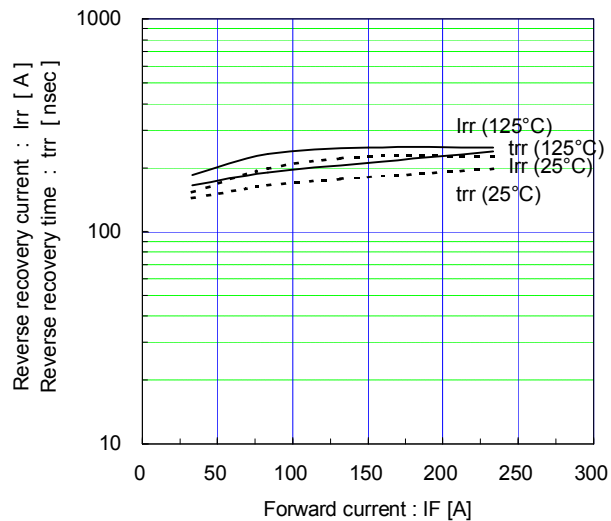
Reverse recovery characteristics (typ.) V_{cc}=900\text{V} , V_{GE}=\pm 15\text{V} , R_g=3.3\Omega
