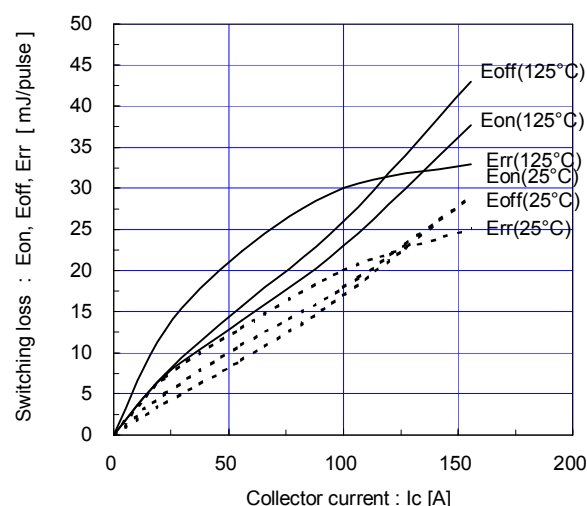
Switching loss vs. Collector current (typ.) Vcc=900V, VGE=±15V, Rg=4.7Ω
