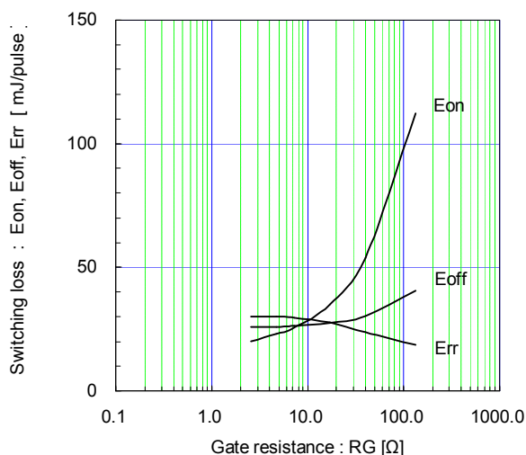
Switching loss vs. Gate resistance (typ.) Vcc=900V, Ic=100A, VGE=±15V, Tj= 125°C
