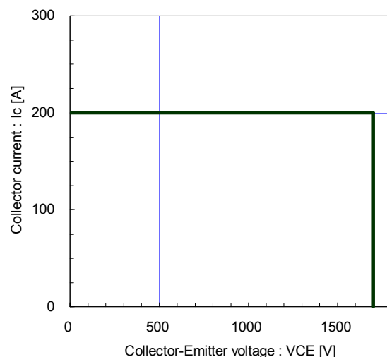
Reverse bias safe operating area (max.) +VGE=15V, -VGE ≤ 15V, Rg ≥ 4.7Ω, Tj ≤ 125°C
