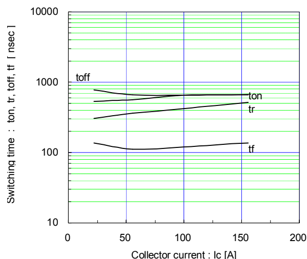
Switching time vs. Collector current (typ.) Vcc=900V, VGE=±15V, Rg=4.7Ω, Tj=125°C
