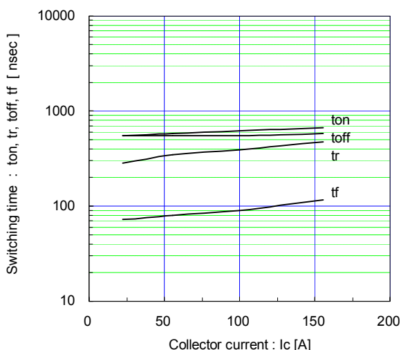
Switching time vs. Collector current (typ.) Vcc=900V, VGE=±15V, Rg=4.7Ω, Tj= 25°C
