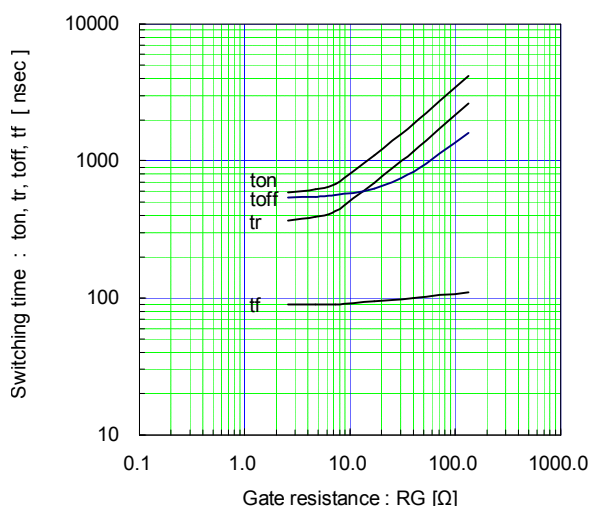
Switching time vs. Gate resistance (typ.) Vcc=900V, Ic=100A, VGE=±15V, Tj= 25°C
