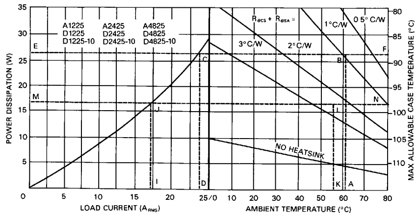
Figure 3. Use of Thermal Derating Curves: 25 Amps, 120, 240 and 480V (Examples.)
