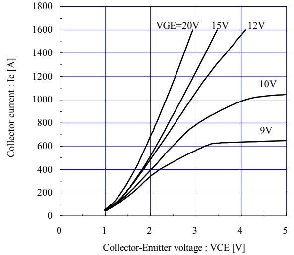
Collector current vs. Collector-Emmitter voltage (typ.) Tj= 125°C, sense terminal
