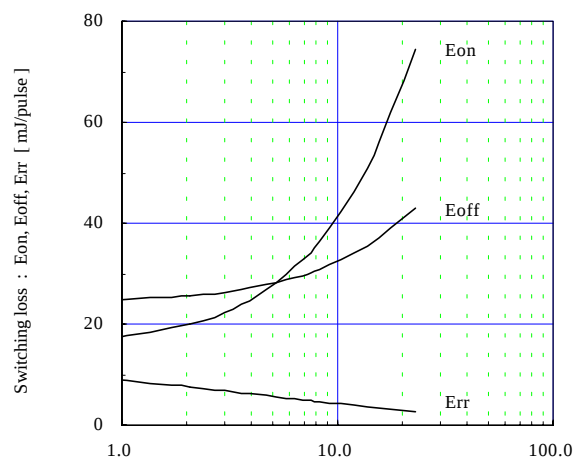
Switching loss vs. Gate resistance (typ.)
