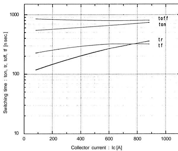
Switching time vs. Collector current V CC =300V, R G =2.7 ohm, V GE =±15V, T J =125°C
