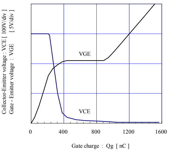
Dynamic Gate charge (typ.) Vcc=300V, Ic=400A, Tj= 25°C
