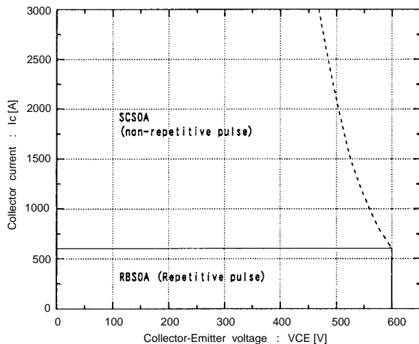
Reversed biased safe operating area +V_{GE}=15V, -V_{GE} \le 15V, T_J \le 125^\circ C, R_G \ge 6.8ohm
