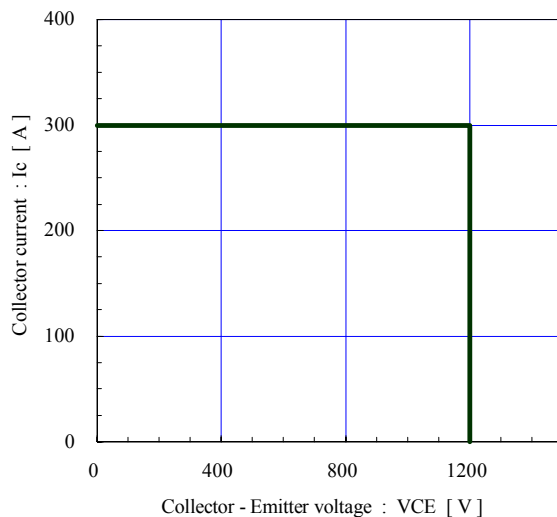
Reverse bias safe operating area (max.) +V_{GE}=15V, -V_{GE} \le 15V, R_g \ge 4.7\Omega, T_j \le 125^\circ C
