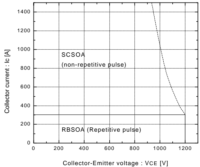
Reversed biased safe operating area +V_{GE}=15V, -V_{GE}\le 15V, T_J\le 125^\circ C, R_G\ge 5.6\Omega
