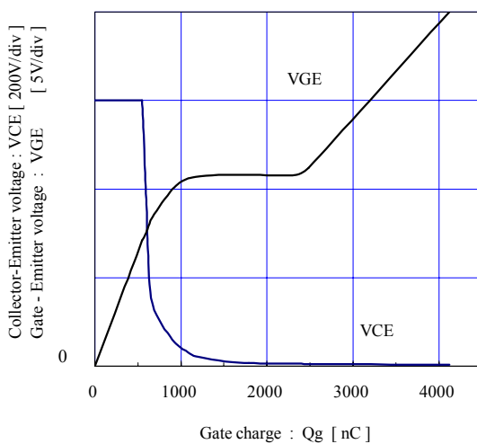
Dynamic Gate charge (typ.)
