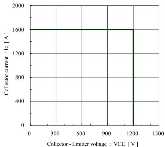
Reverse bias safe operating area (max.) +V_{GE}=15V, -V_{GE} \leq 15V, R_g \geq 0.68\Omega, T_j \leq 125^\circ C
