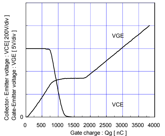
Dynamic Gate charge (typ.) Vcc=600V, Ic=800A, Tj=25°C
