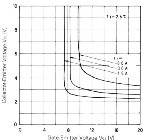
Collector-Emitter Voltage vs. Gate-Emmitter Voltage
