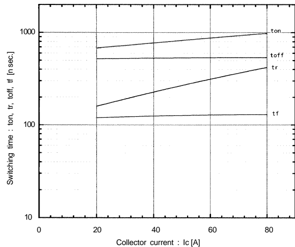
Switching time vs. Collector current Vcc=300V, Rg=62 ohm, VGE=±15V, Tj=25°C
