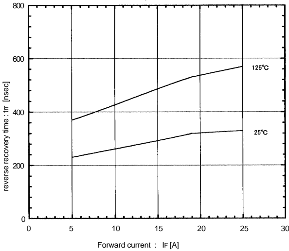
Reverse recovery time vs. Forward current -di/dt=45A / \mu sec
