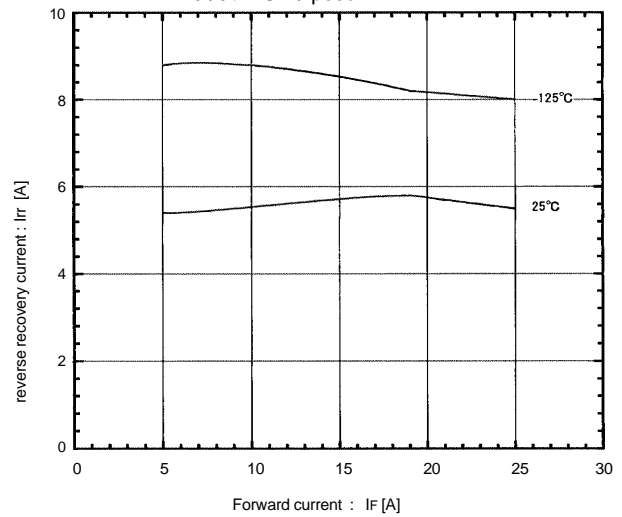
Reverse recovery current vs. Forward current -di/dt=45A / \mu sec
